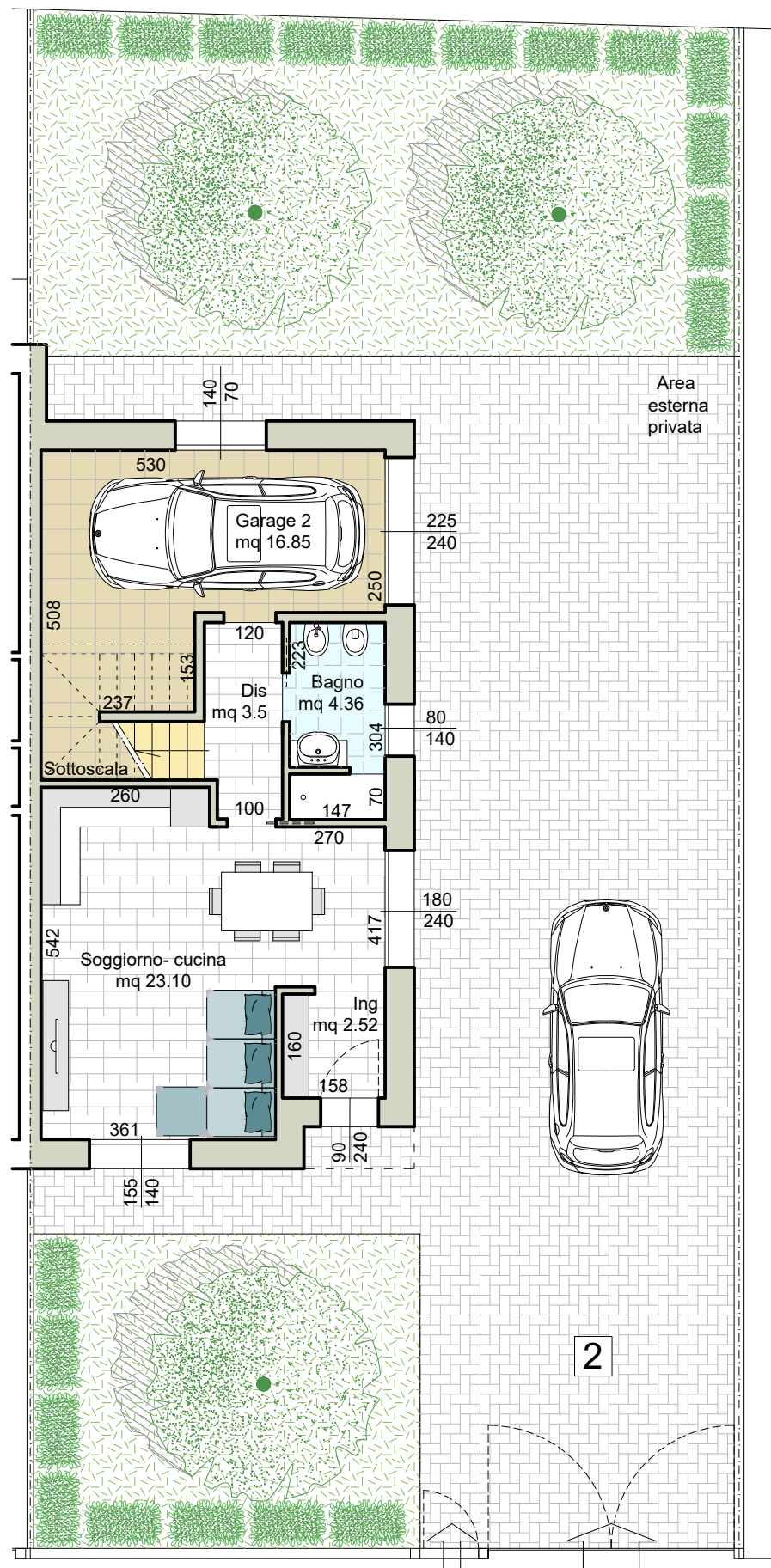
Piano terra
